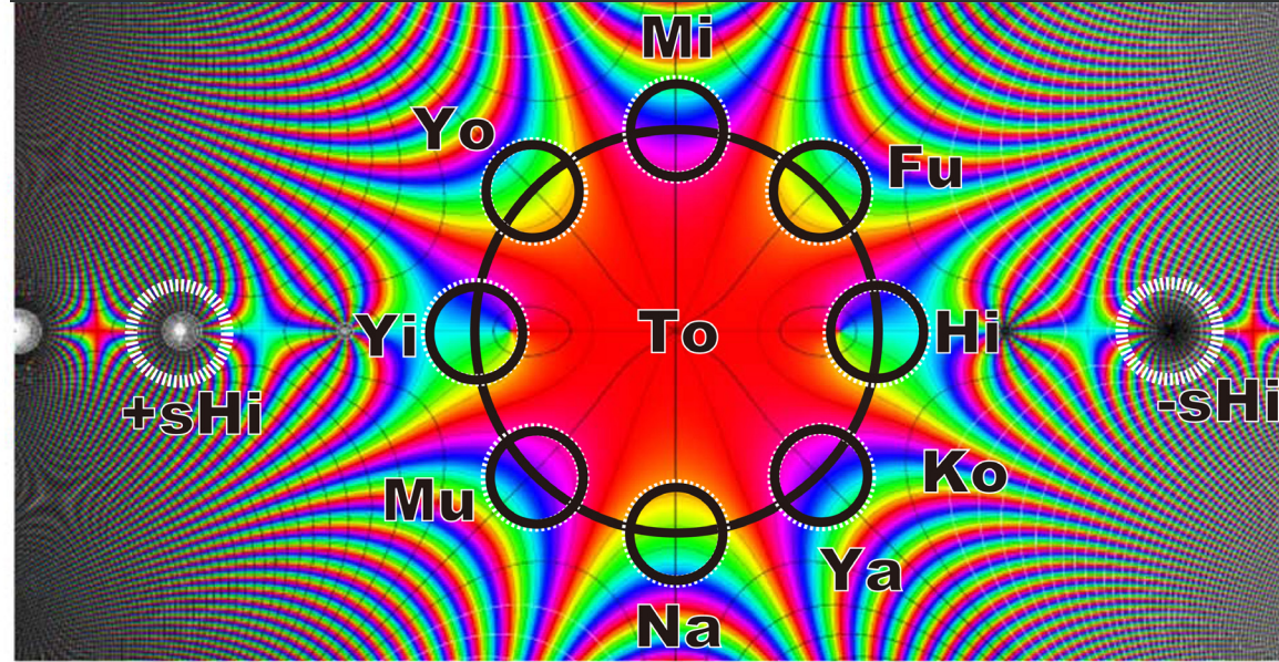
fig ; background image is Graph of multiple trigonometric functions of Kurokawa of complex variables ; http://math-functions-1.watson.jp/sub1_spec_010.html Copyright Souichiro-Ikebe
