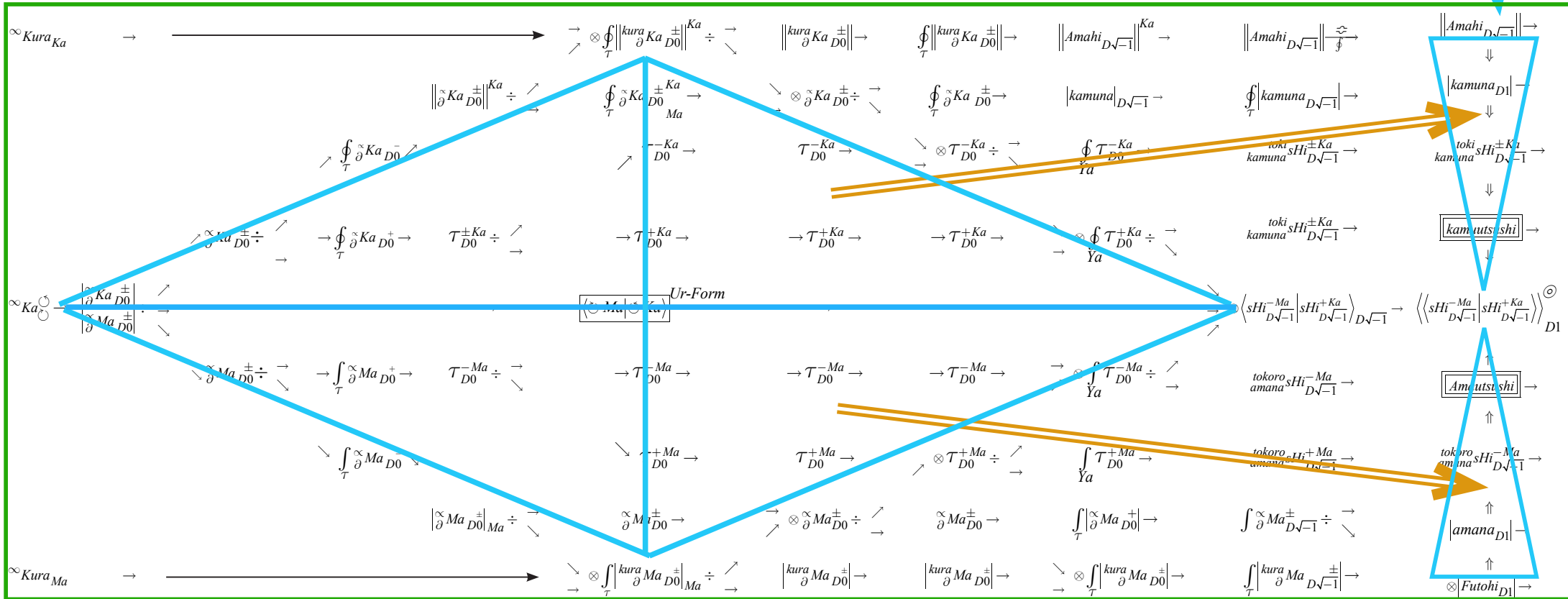
Definition area of "Axiom K"
